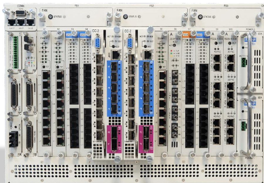
ETSI Front View of HX9800
